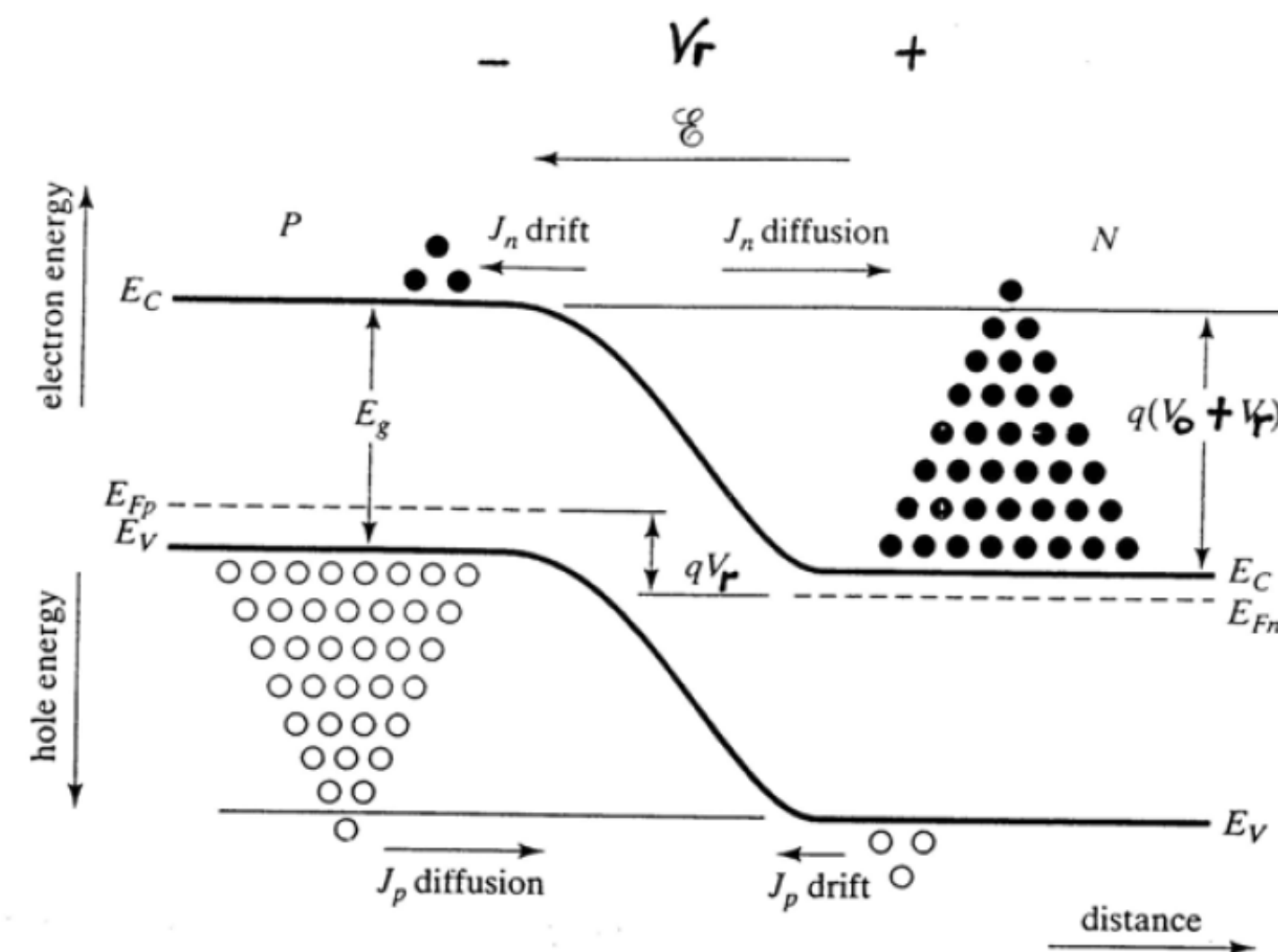
Reverse Bias
