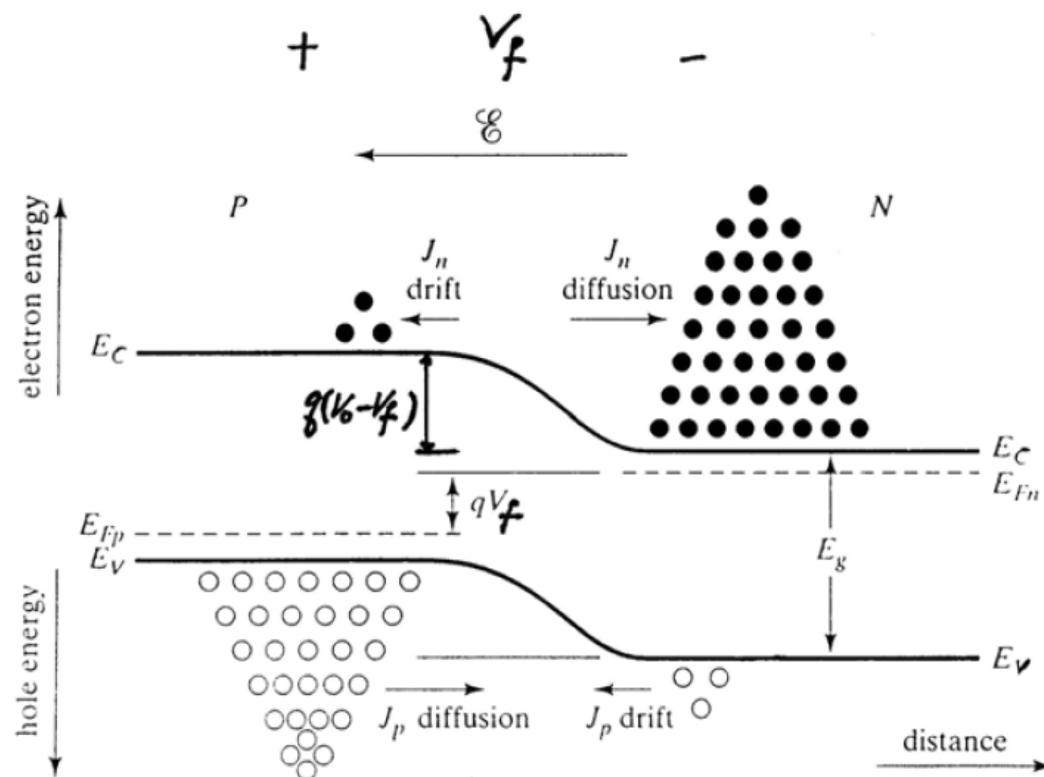
Forward Bias
